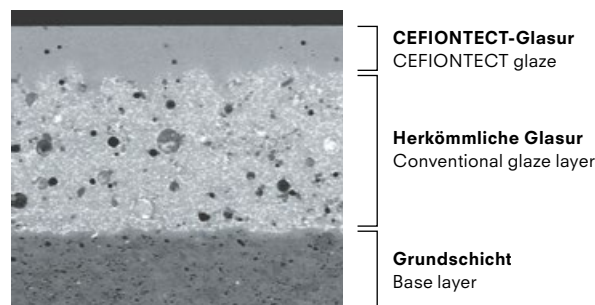
CEFIONTECT WC-Mikrograph * 1 µm=0,001 mm CEFIONTECT toilet micrograph * 1 µm=0.001 mm
